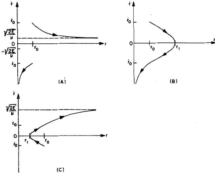
Fig. 1. Coulomb's law. (A) \alpha < 0 , and E \geq 0 ; (B) \alpha < 0 and E < 0 ; (C) \alpha > 0 , E > 0 .
